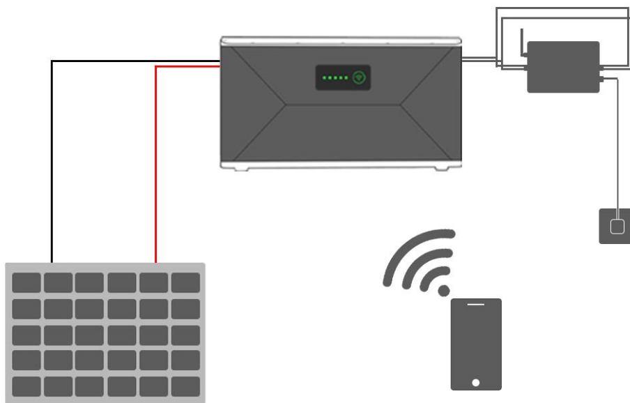
SF100 Working Principle Diagram
